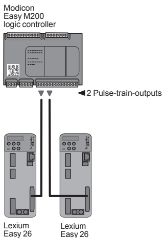
Example of architecture with control by Modicon Easy M200 logic controller
