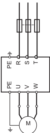
LXM26 servo drive, BCH2 servo motor with fuse protection
