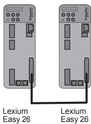
Example of a Lexium Easy 26 drive controlling another Lexium Easy 26 drive with PTI/ESIM interfaces
