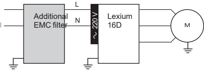
Lexium 16D servo drive with additional EMC filter
